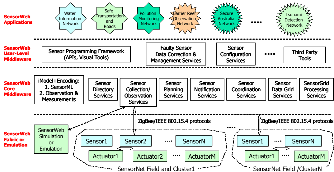
Figure 3 – Open SensorWeb Architecture.
