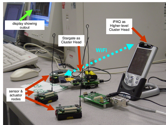
Figure 2 – Hierarchical decision fusion system on sensor-grid architecture.
