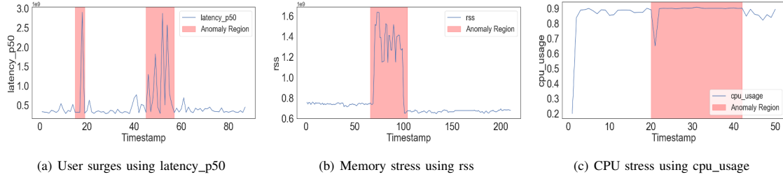
Fig. 12. Visualization of selected anomalies from the dataset
