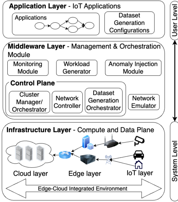
Fig. 1. System architecture of iAnomaly
