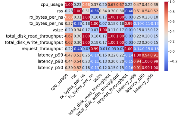
Fig. 9. Collinearity among metrics in the generated dataset
