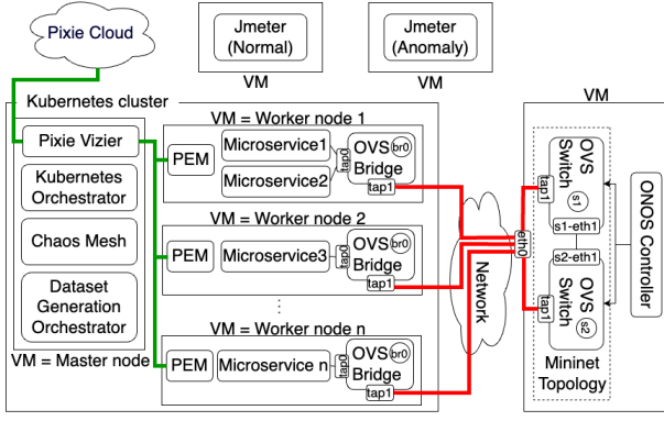
Fig. 2. Deployment diagram of the iAnomaly toolkit
