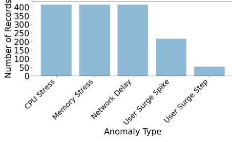
Fig. 8. Distribution of records by anomaly type
