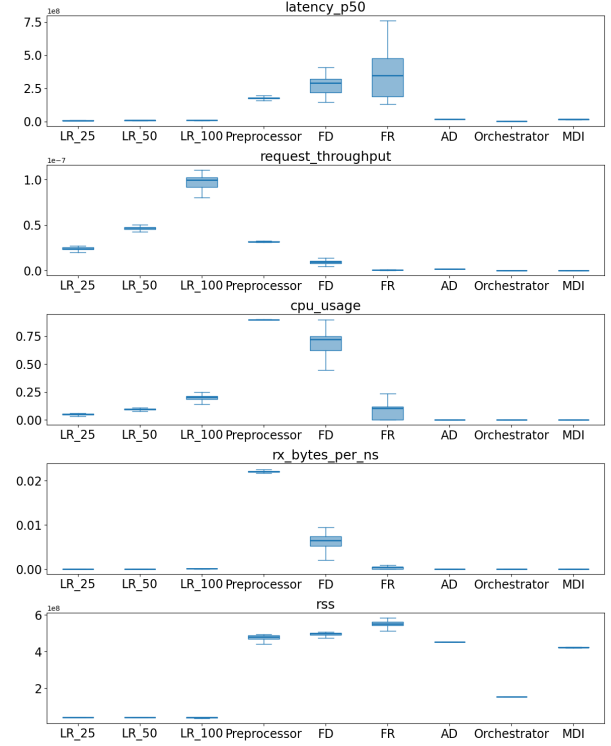
Fig. 10. Distribution of normal data across shortlisted metrics
