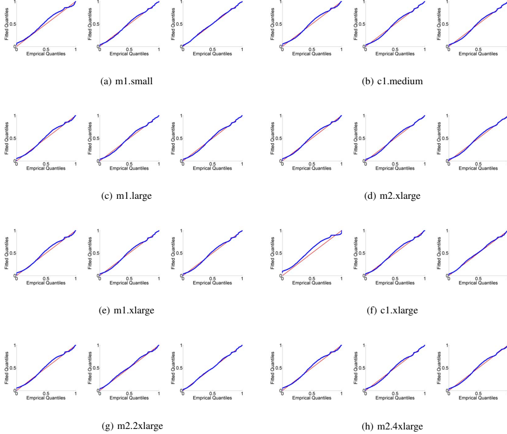
Fig. 6. PP-plots of the inter-price time in eu-west for mixture of Gaussians ( k = 2, k = 3, k = 4 ). X-axis: empirical quantiles, and Y-axis: fitted quantiles.
