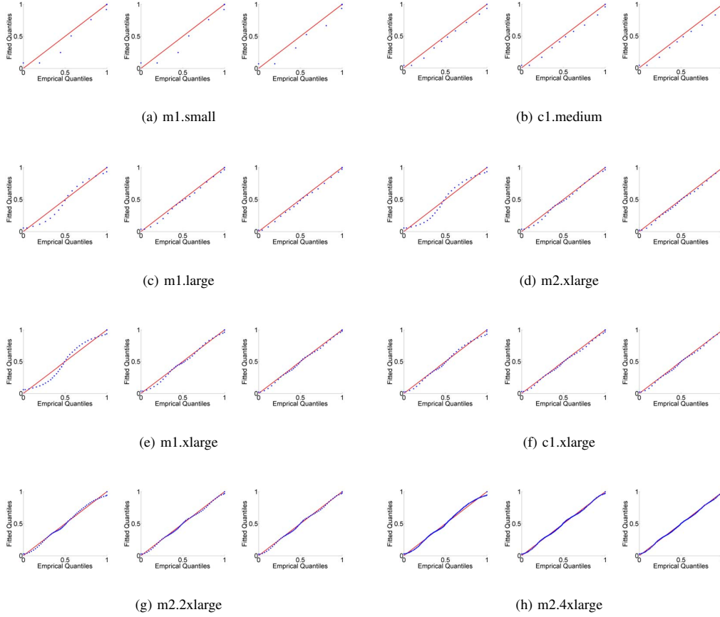
Fig. 5. PP-plots of spot price in eu-west for mixture of Gaussians ( k = 2, k = 3, k = 4 ). X-axis: empirical quantiles, and Y-axis: fitted quantiles.
