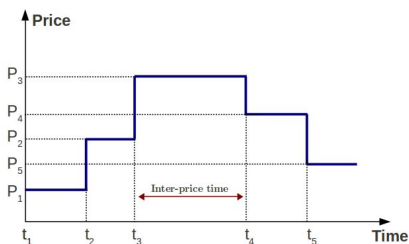
Fig. 1. Spot price and the inter-price time of Spot instances.
