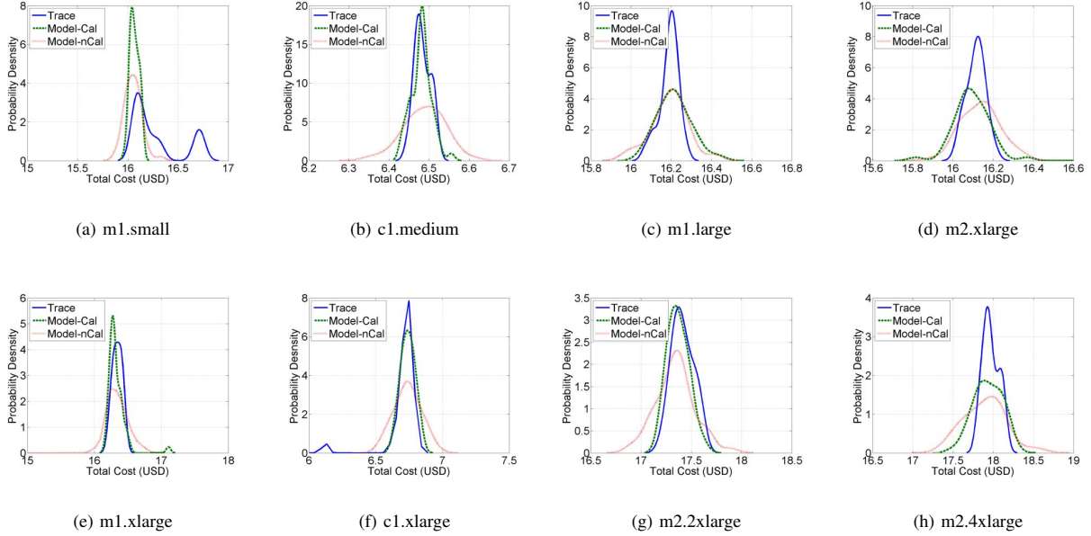
Fig. 9. Model validation for all SIs in eu-west for the new traces (Dec-2010 to mid-Feb-2011).
