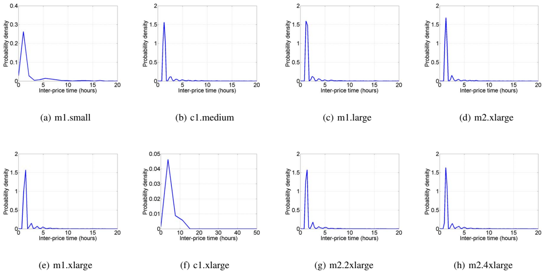
Fig. 4. Probability density functions of the inter-price time for all SIs in eu-west data center.
