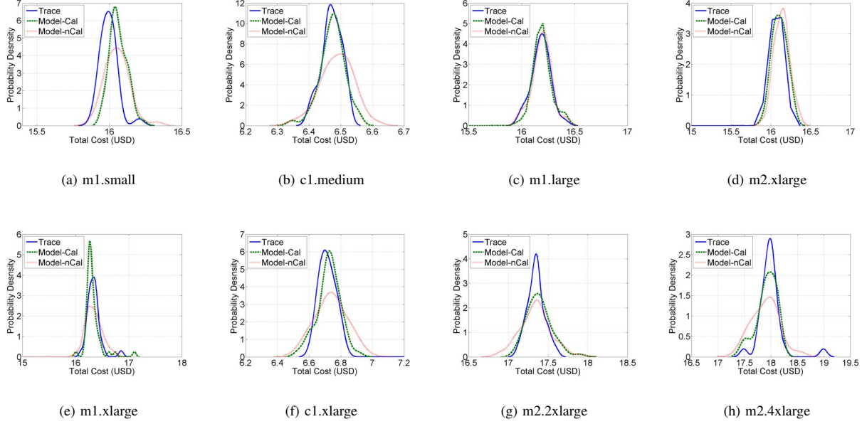
Fig. 8. Model validation for all SIs in eu-west for the modeling traces (Feb-2010 to Nov-2010).
