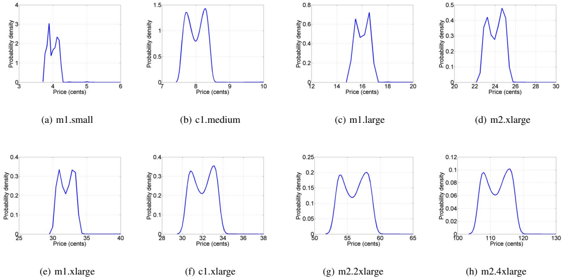
Fig. 3. Probability density functions of spot price for all SIs in eu-west data center.
